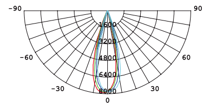
Light Distribution Curve
