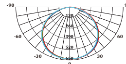
Light Distribution Curve
