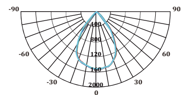
Light Distribution Curve
