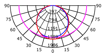
Light Distribution Curve
