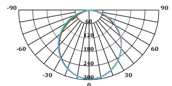
Light Distribution Curve
