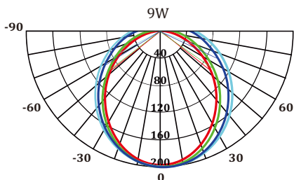
Light Distribution Curve
